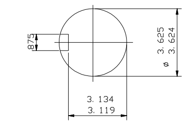
ENLARGED VIEW OF SHAFT EXTENSION
